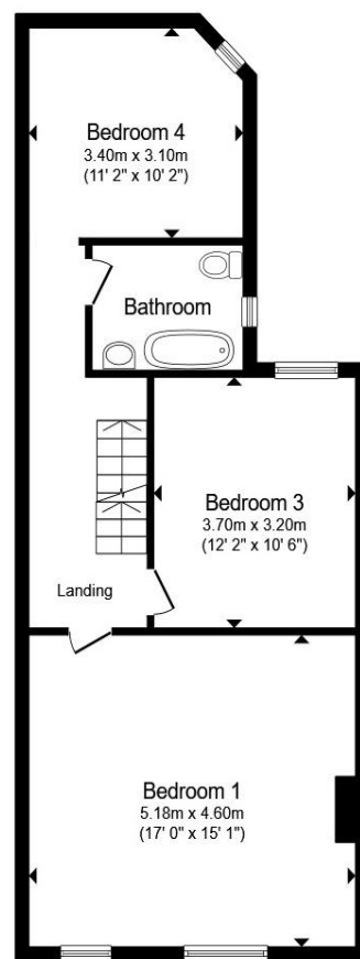
First Floor
