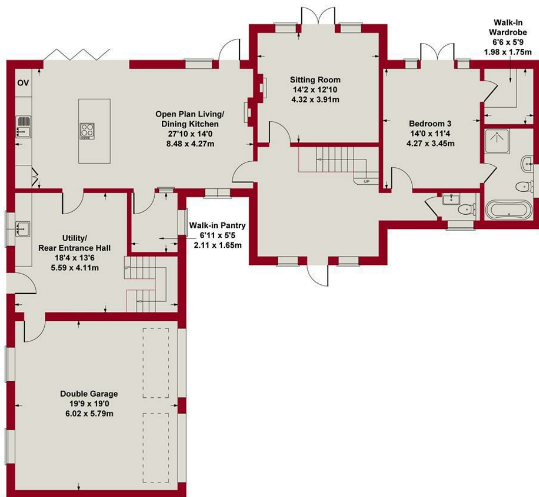
GROUND FLOOR
