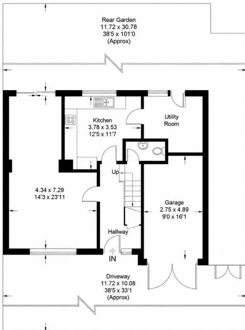
Ground Floor
