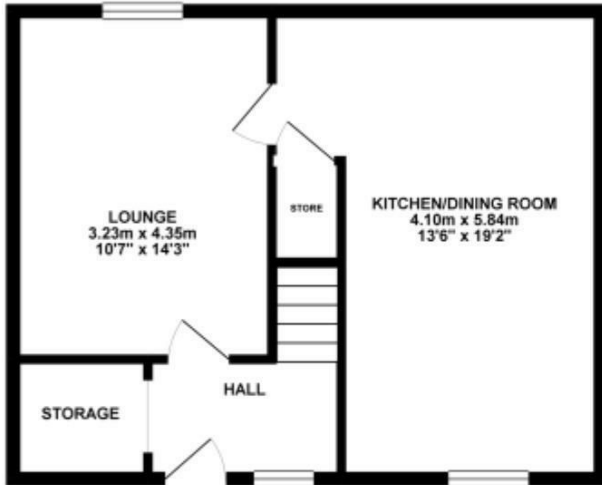
GROUND FLOOR 42.85 sq. m. ( 461.21 sq. ft. )
