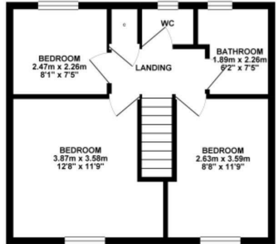
1ST FLOOR 38.03 sq. m. ( 409.32 sq. ft. )
