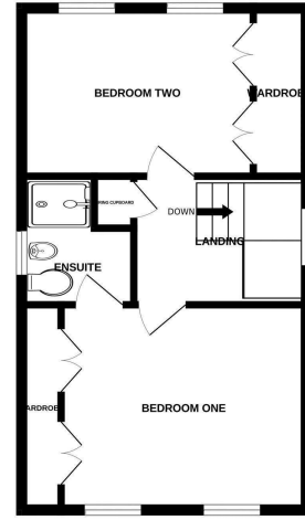
2ND FLOOR 404 sq.ft. (37.5 sq.m.) approx.
