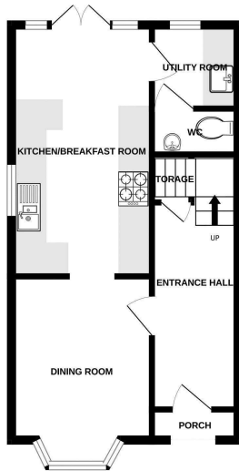
GROUND FLOOR 399 sq.ft. (37.1 sq.m.) approx.
