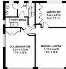
POOL COTTAGE GROUND FLOOR (ANNEXE)
