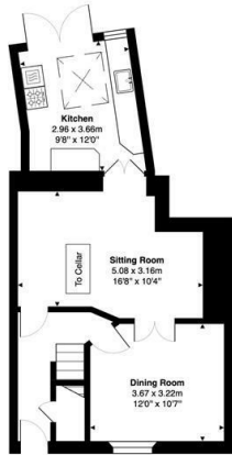
Ground Floor Gross Internal Area: 47.7 m 2 ... 513 ft 2
