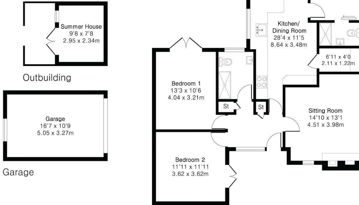
Ground Floor
