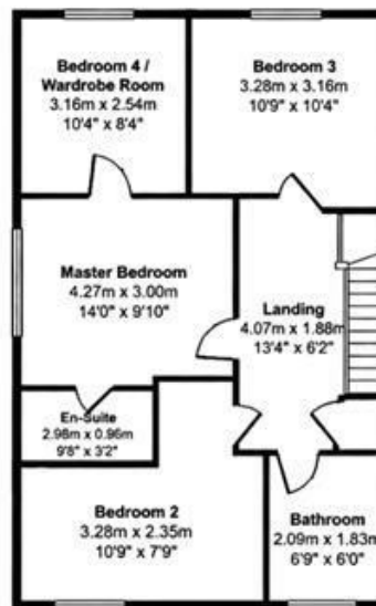
First Floor Approx 48 sq m / 517 sq ft
