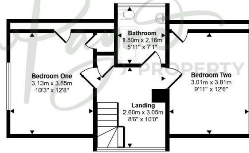
First Floor Approx 40 sq m / 435 sq ft
