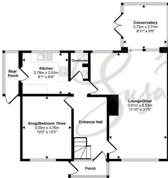
Ground Floor Approx 71 sq m / 768 sq ft
