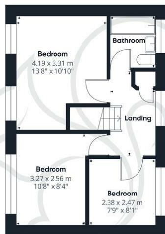
Floor 1
