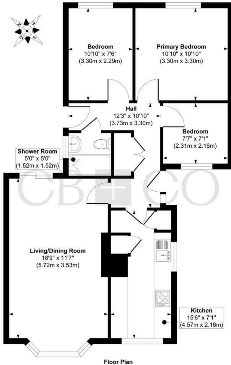
Floor Plan
