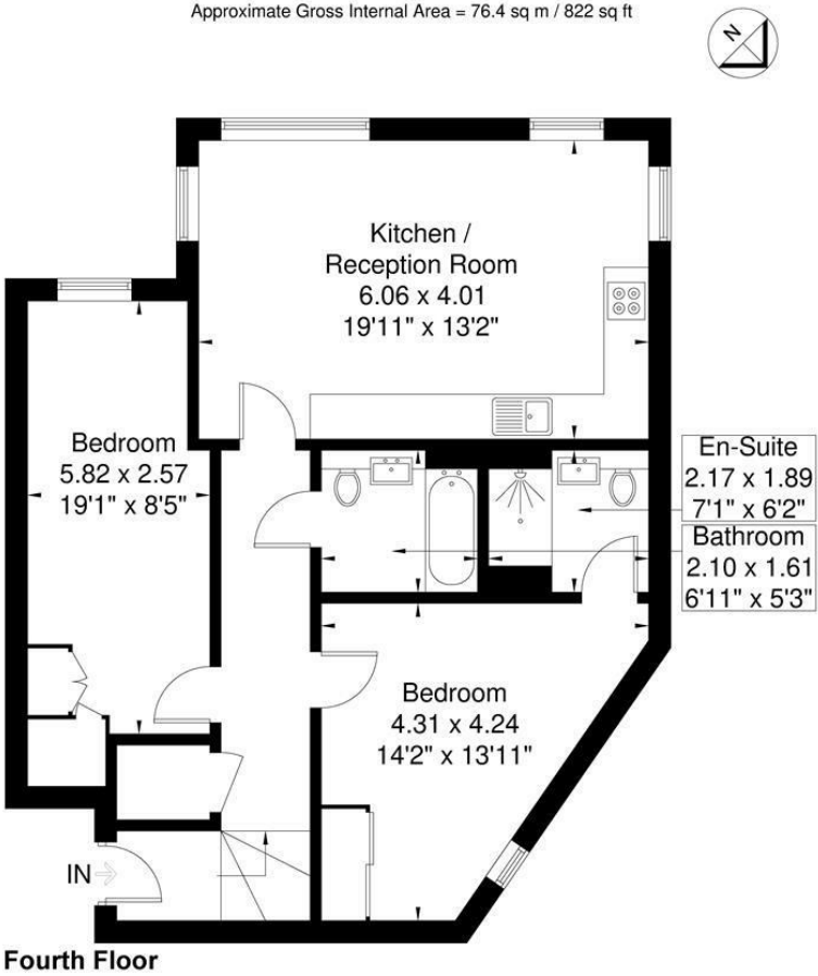
Acton Town Hall Approximate Gross Internal Area = 76.4 sq m / 822 sq ft
