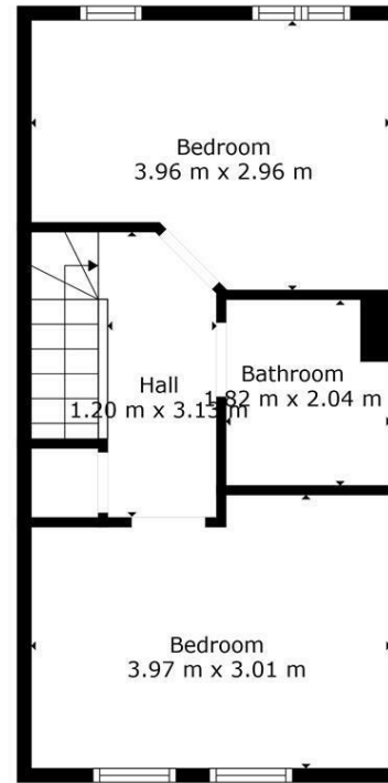
Floor 3
