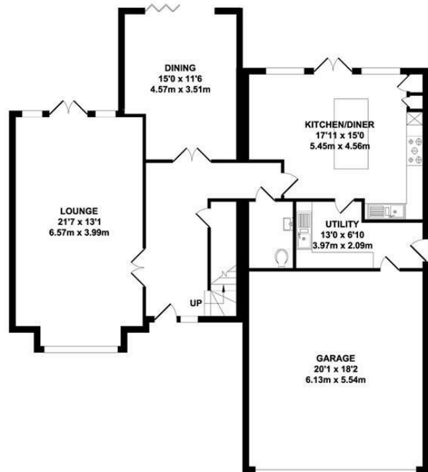
GROUND FLOOR APPROX. FLOOR AREA 1374 SQ.FT. (127.69 SQ.M.)
