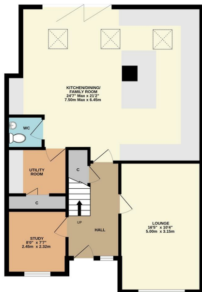
GROUND FLOOR 820 sq.ft. (76.2 sq.m.) approx.
