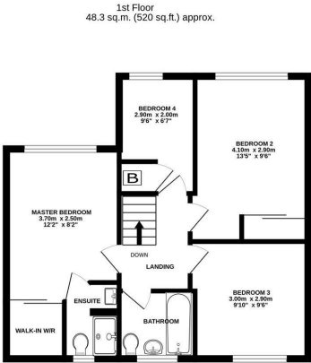
TOTAL FLOOR AREA : 96.6 sq.m. (1040 sq.ft.) approx. Whilst every attempt has been made to ensure the accuracy of the floorplan contained here, measurements of doors, windows, rooms and any other items are approximate and no responsibility is taken for any error, omission or mis-statement. This plan is for illustrative purposes only and should be used as such by any prospective purchaser. The services, systems and appliances shown have not been tested and no guarantee as to their operability or efficiency can be given. Made with MetreX v2024
