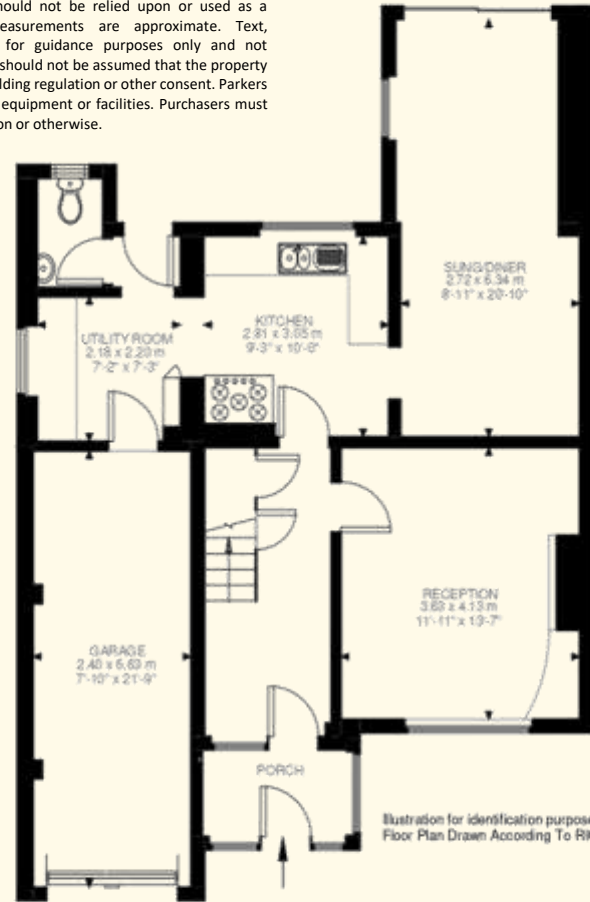
Ground Floor 686 ft²
