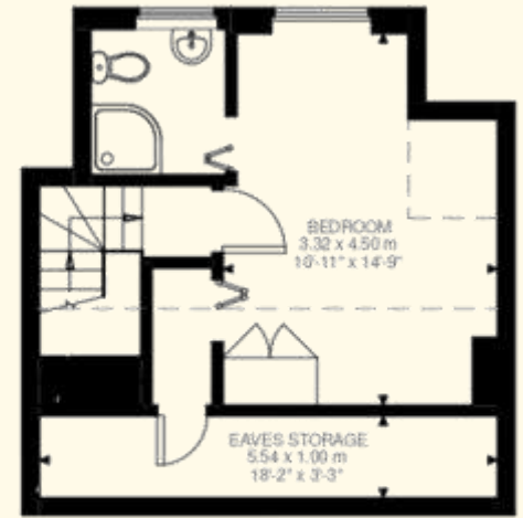
Second Floor 248 ft²
