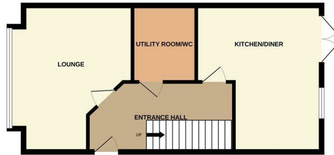
GROUND FLOOR 513 sq.ft. (47.6 sq.m.) approx.
