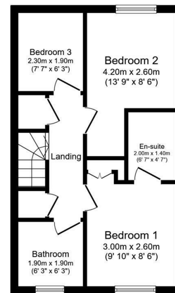
First Floor Floor area 36.8 sq.m. (396 sq.ft.)
