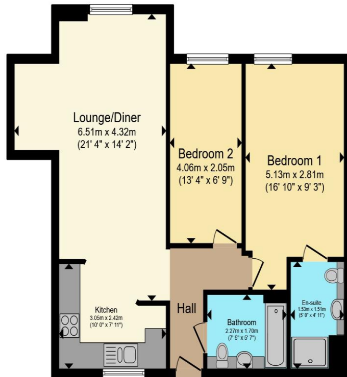
Floor Plan
