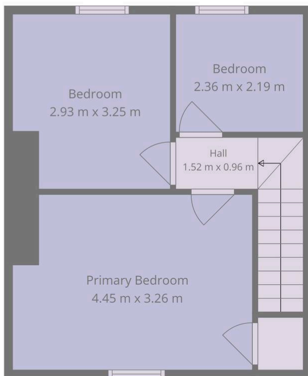
1st Floor
