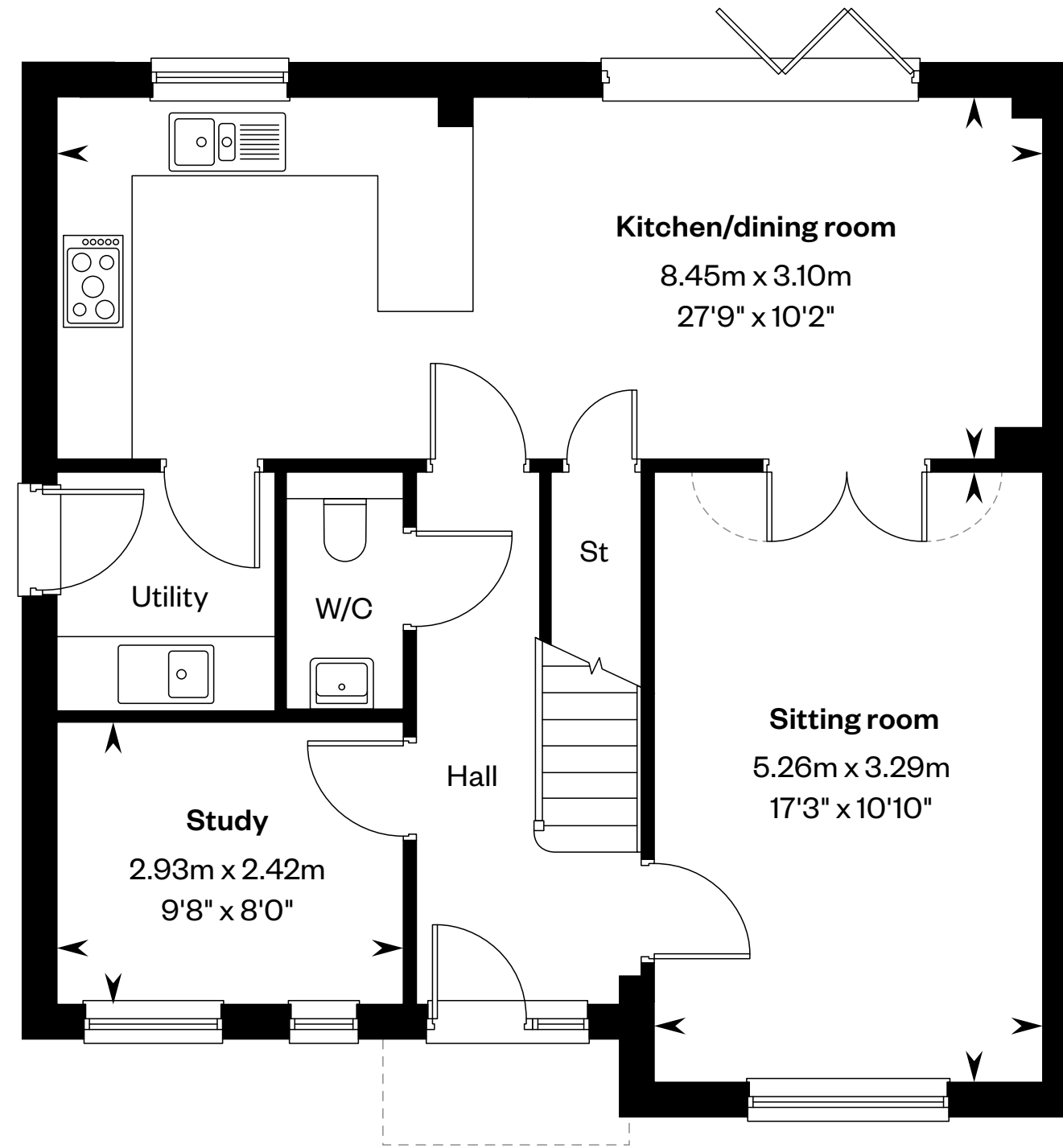
Ground floor
