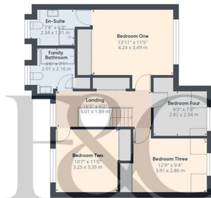
Floor 1 Building 1
