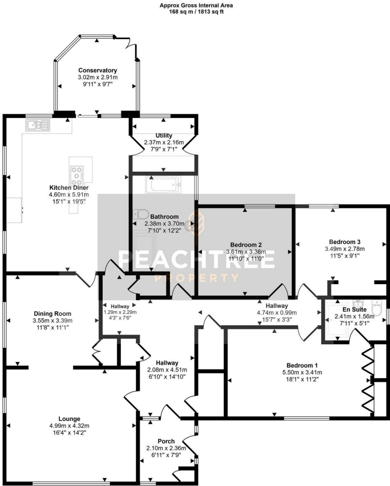
Floorplan
