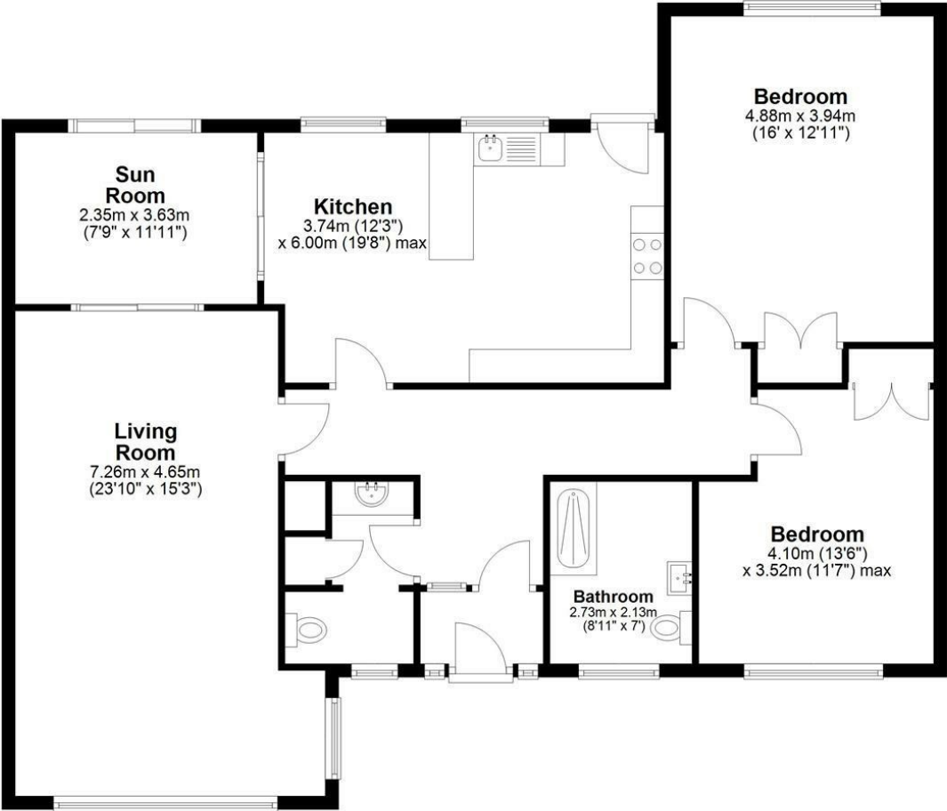
Total area: approx. 124.7 sq. metres (1342.4 sq. feet) The Lindens, Woodfall Lane, Little Neston, NESTON
