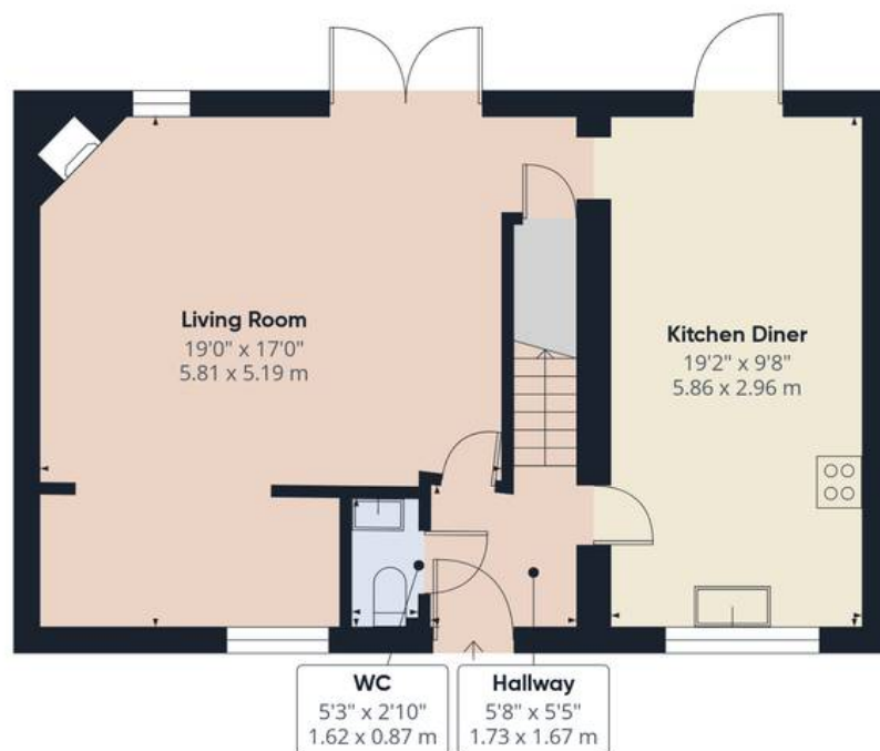
Floor 1 Building 1
