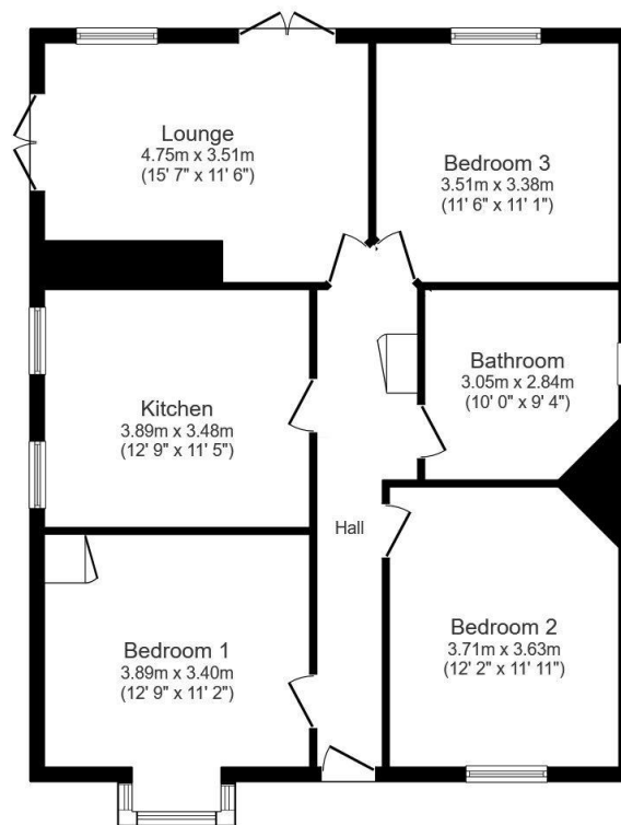
Floor Plan
