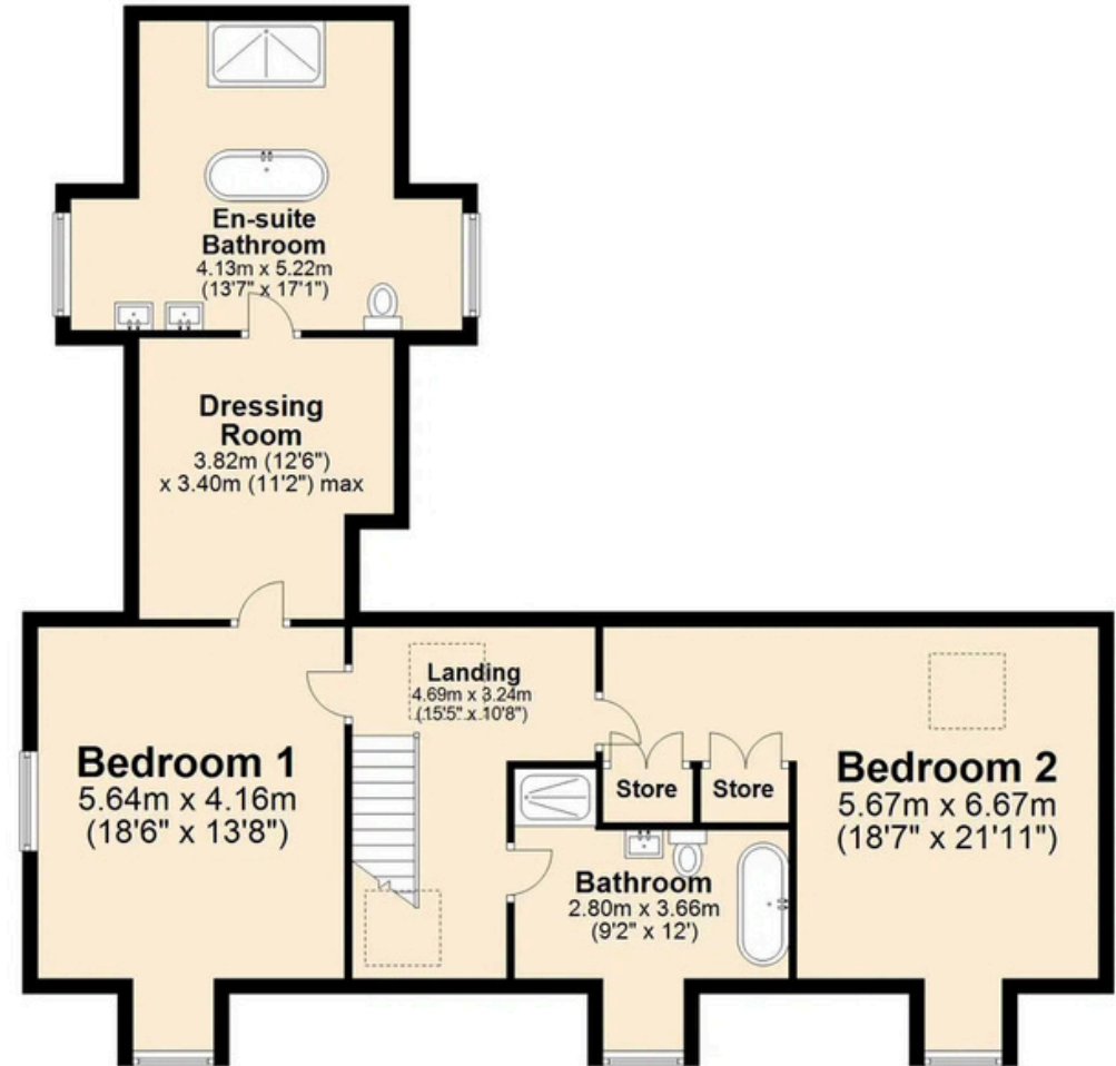
First Floor Approx. 99.3 sq. metres (1068.9 sq. feet)
