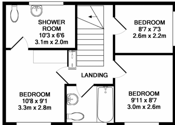
1ST FLOOR APPROX. FLOOR AREA 415 SQ.FT. (38.6 SQ.M.)
