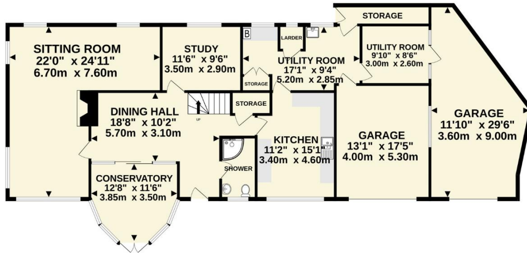
GROUND FLOOR 1892 sq.ft. (175.7 sq.m.) approx.
