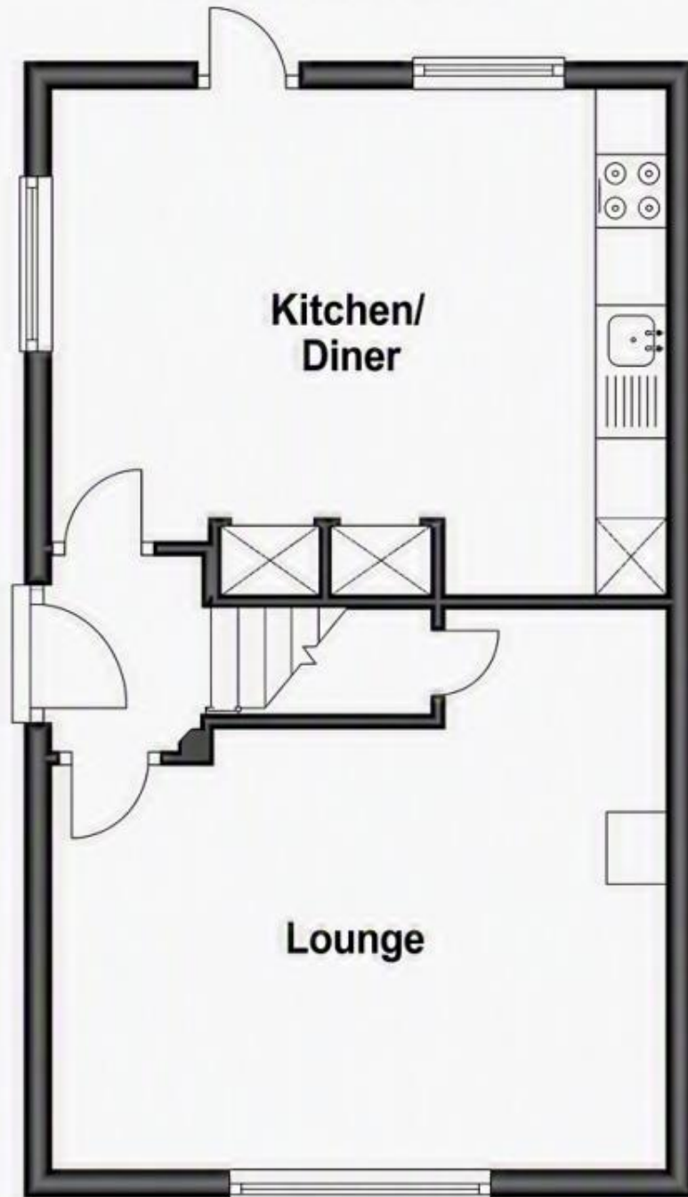
Ground Floor
