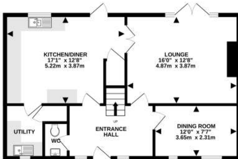
GROUND FLOOR 663 sq.ft. (61.6 sq.m.) approx.
