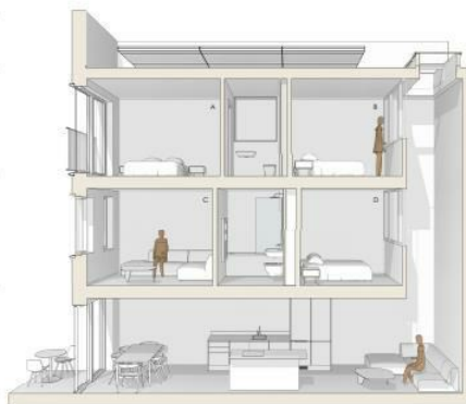
SECTION 1:50
