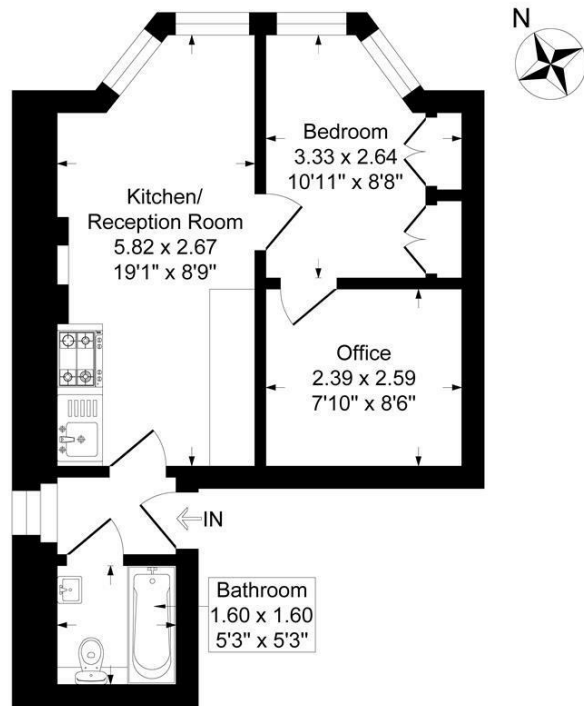
Second Floor
