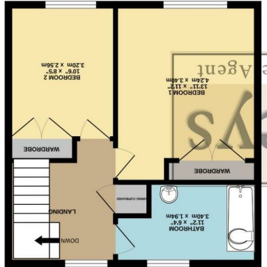
1ST FLOOR (36.8 sq.m.) approx.
