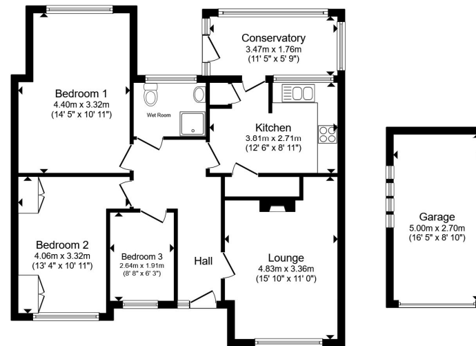
Floor Plan
