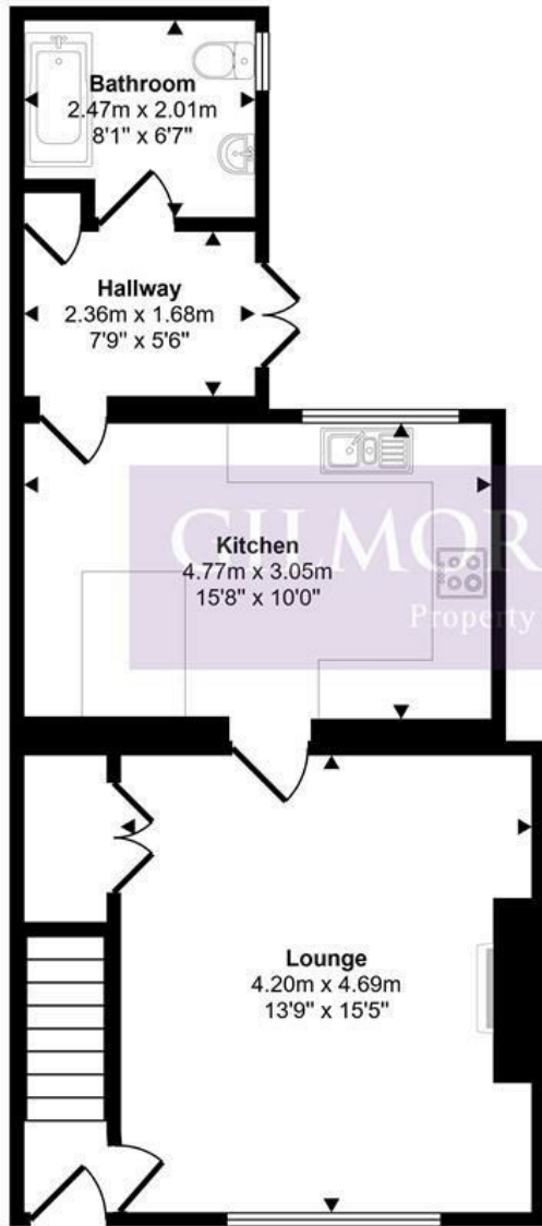
Ground Floor Approx 51 sq m / 549 sq ft
