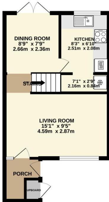
GROUND FLOOR 347 sq.ft. (32.2 sq.m.) approx.
