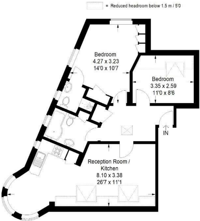
Third Floor
