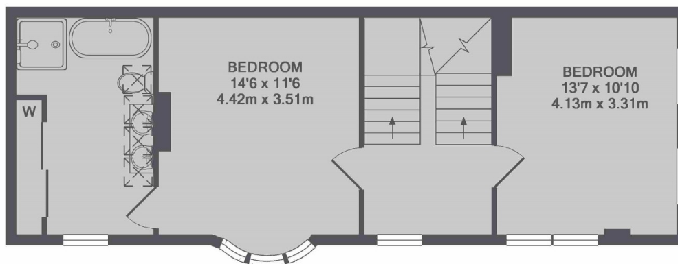
1ST FLOOR
