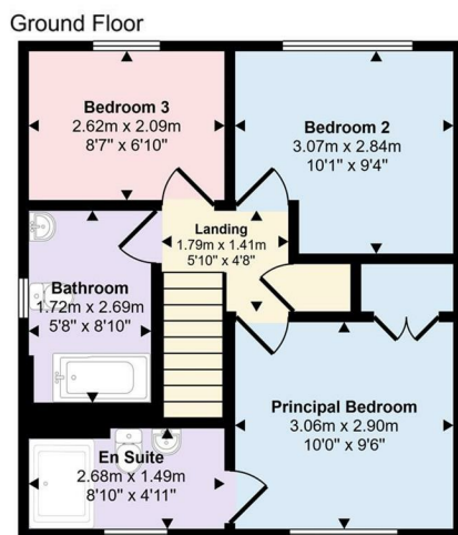
First Floor Approx 40 sq m / 426 sq ft
