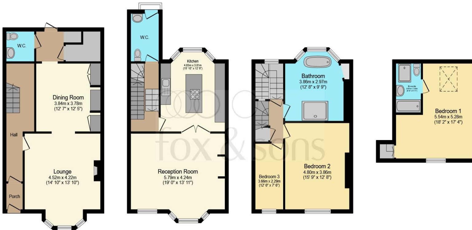
Ground Floor
