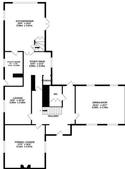
GROUND FLOOR 2092 sq.ft. (194.4 sq.m.) approx.
