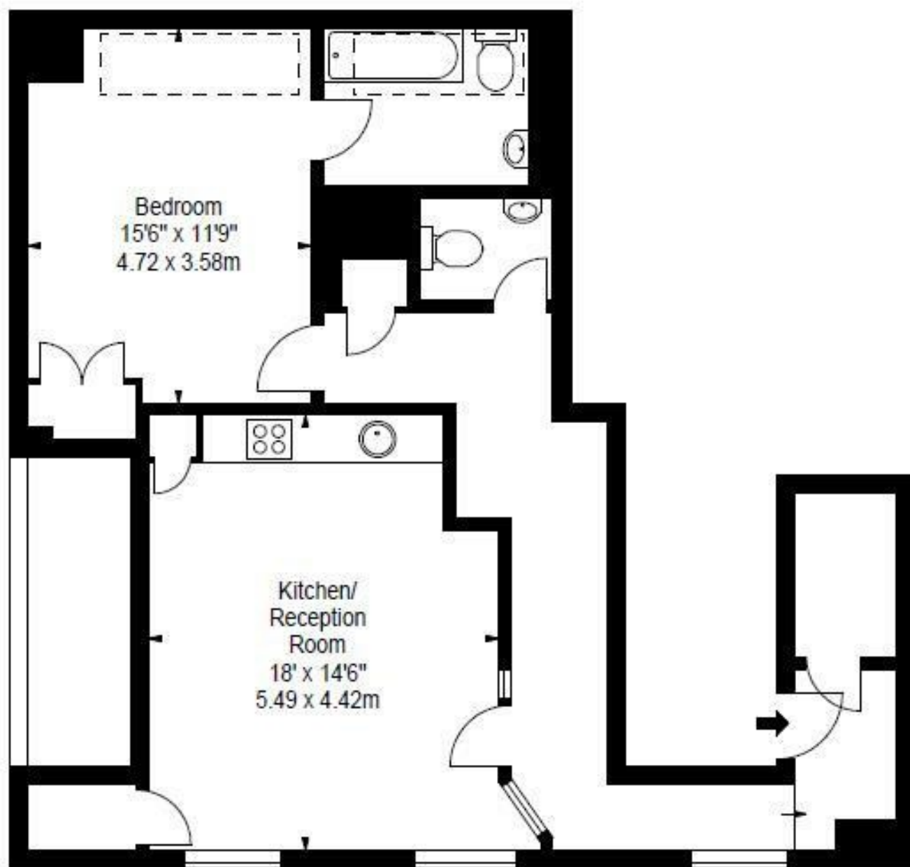
FIRST FLOOR
