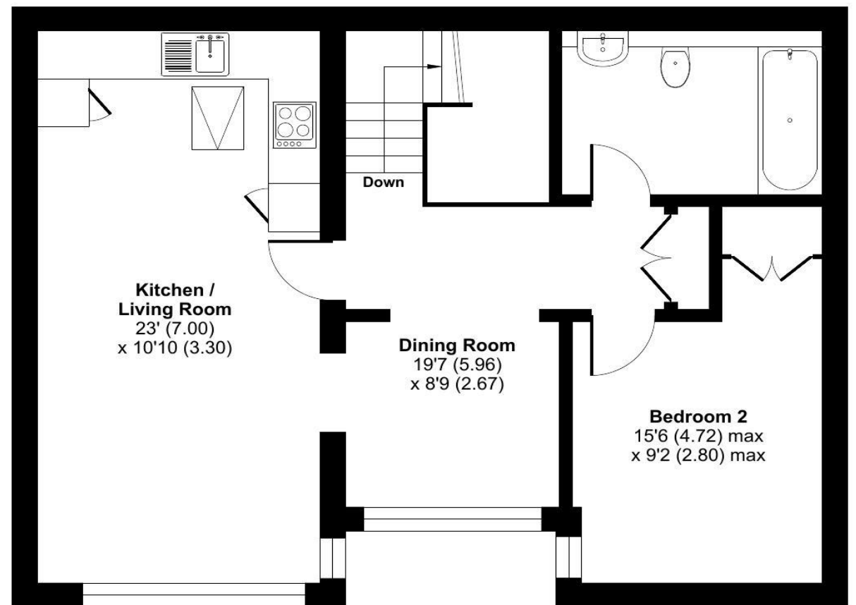
FIRST FLOOR
