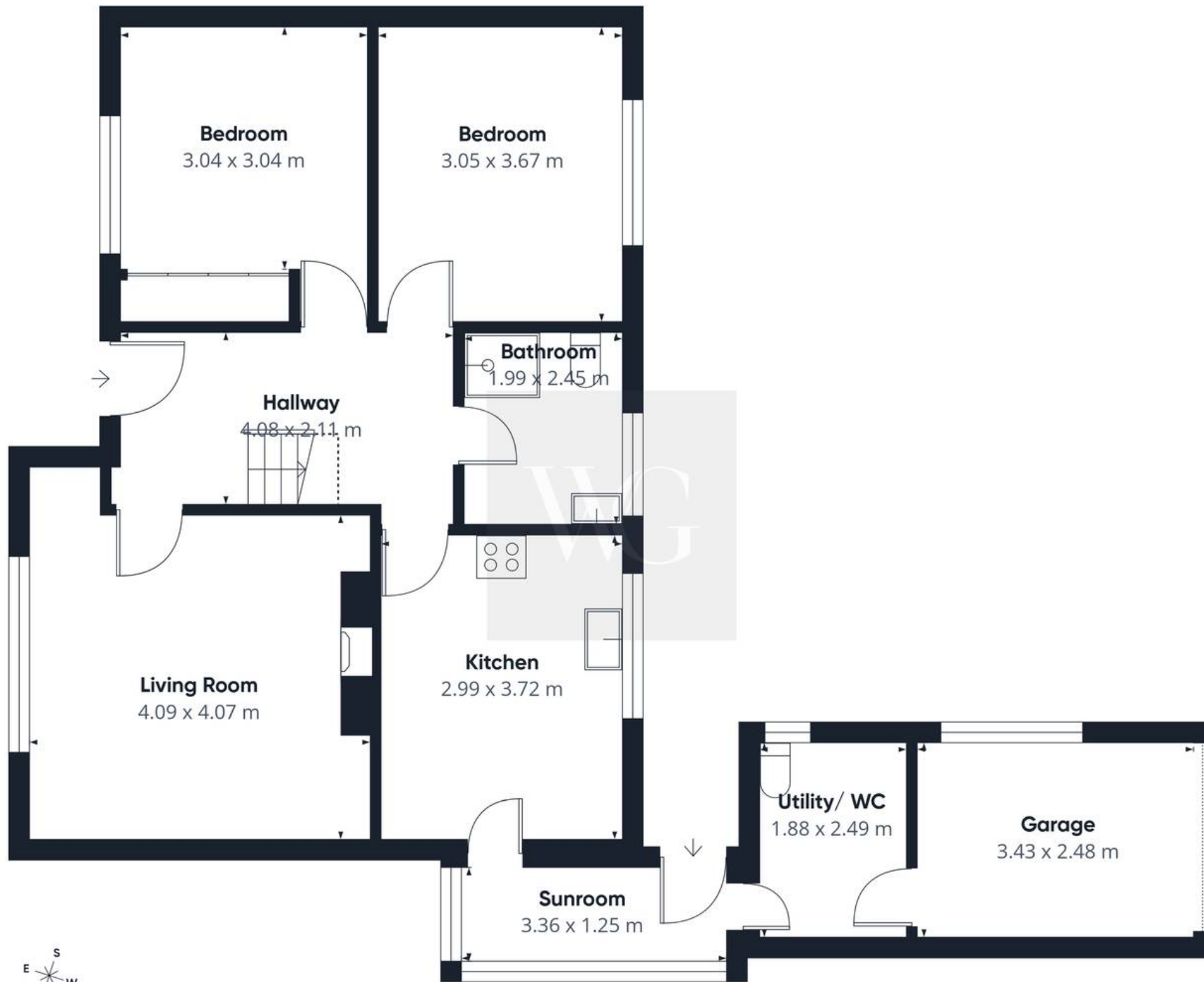
Floor 1
