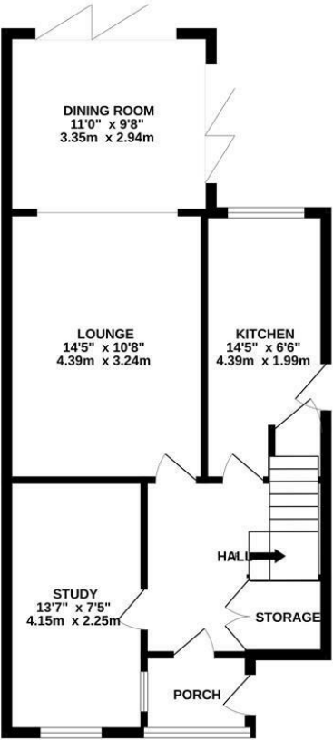
GROUND FLOOR 570 sq.ft. (52.9 sq.m.) approx.
