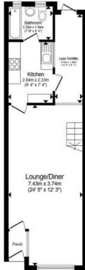
Ground Floor
