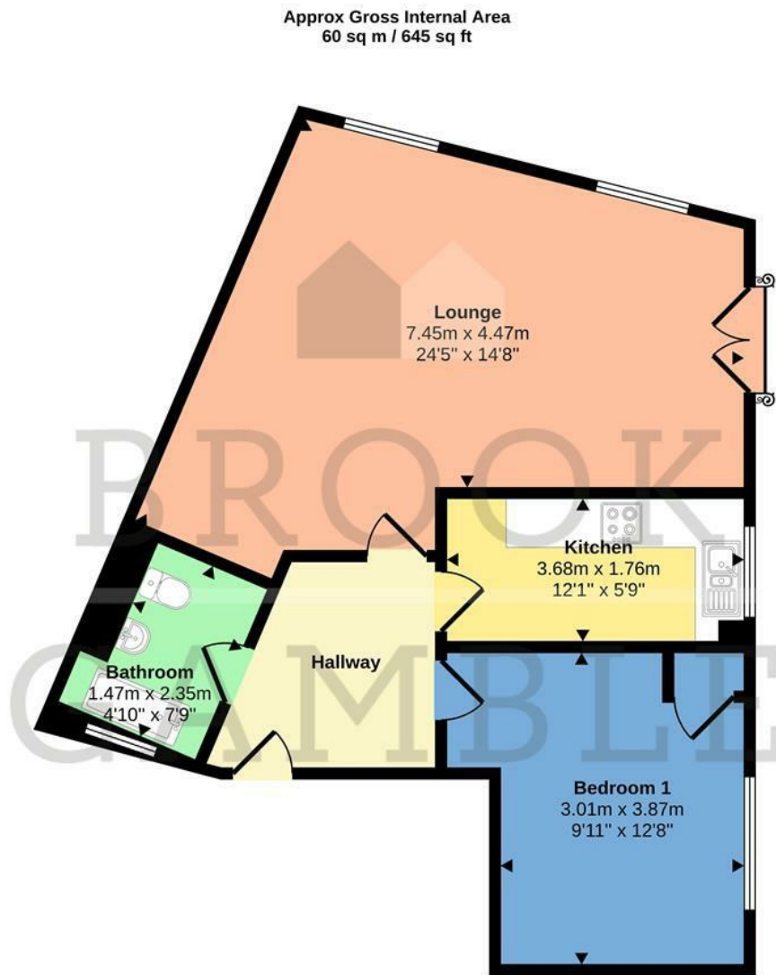
Floorplan
